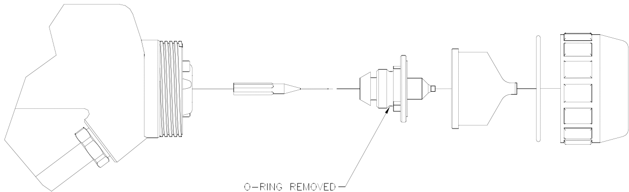
Figure 1 SOLO R90/R70 O-RING REMOVED DIAGRAM
